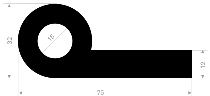
214.00.866 EPDM 70° Shore black roll length 20 meter
