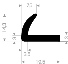
216.51.914 EPDM 70° Shore black roll length 50 meter
