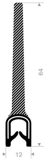
245.00.890 pvc + Solid rubber clamping range 1,5-4 mm roll length 40 meter
