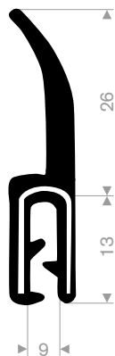
245.00.875 EPDM Solid rubber clamping range 1,5-4 mm roll length 30 meter
