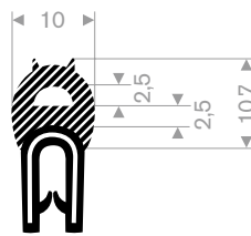
245.00.830 pvc + Sponge rubber clamping range 1-2 mm roll length 50 meter
