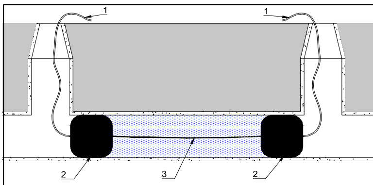
Picture 1: Strutting with steel chain
